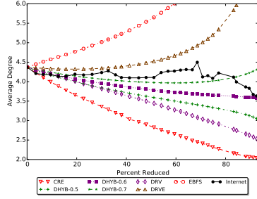
(a) Routeviews 2014-1998
