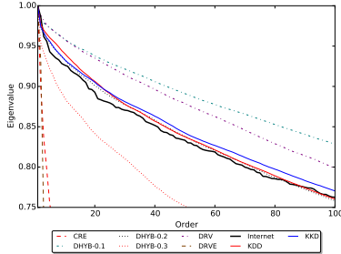
(a) Spectra
