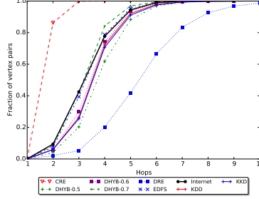
(b) Hop-plot
